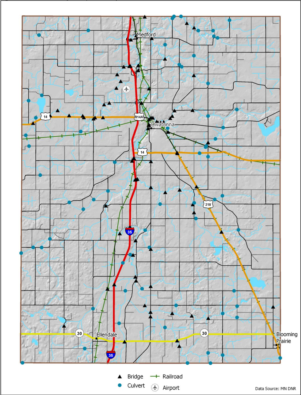
Figure A - 6. Steele County Transportation Infrastructure
